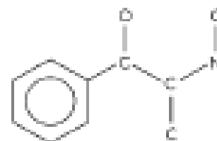
ephedrine
