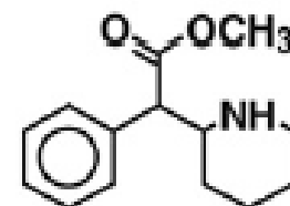
Methylphenidate
