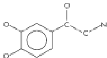
norepinephrine
