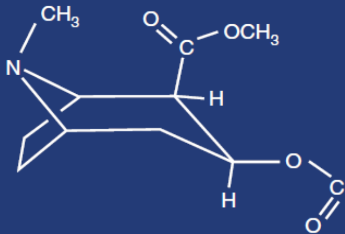
Cocaine
