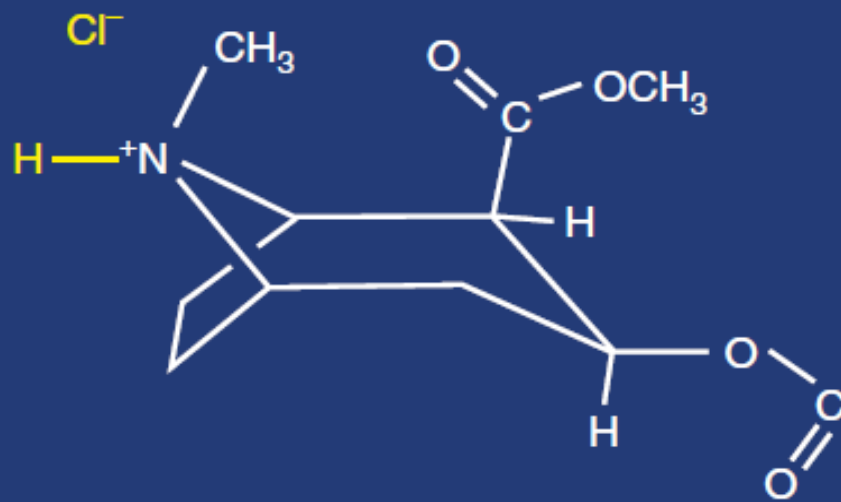
Cocaine Hydrochloride
