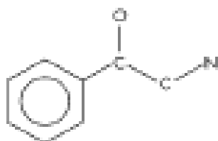
phenylethanolamine
