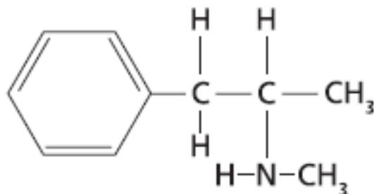
d-methamphetamine
