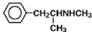
Methamphetamine
