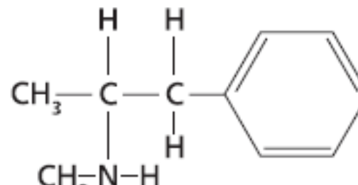
Desoxyephedrine l-methamphetamine
